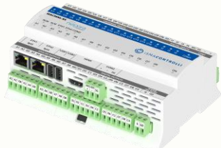
iSMA-B-MAC36NL-M (1xRS485+1xM-Bus)
