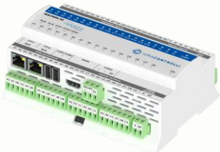
iSMA-B-MAC36NL-M (1xRS485+1xM-Bus)
